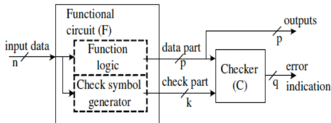
Fig .4 General structure of self-checking circuit
