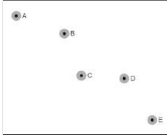
Figure: A discrete data set
