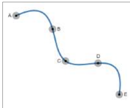
Figure: Example of Interpolation
