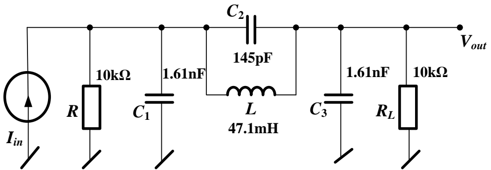
Fig. 3: 25 kHz LC ladder filter.
