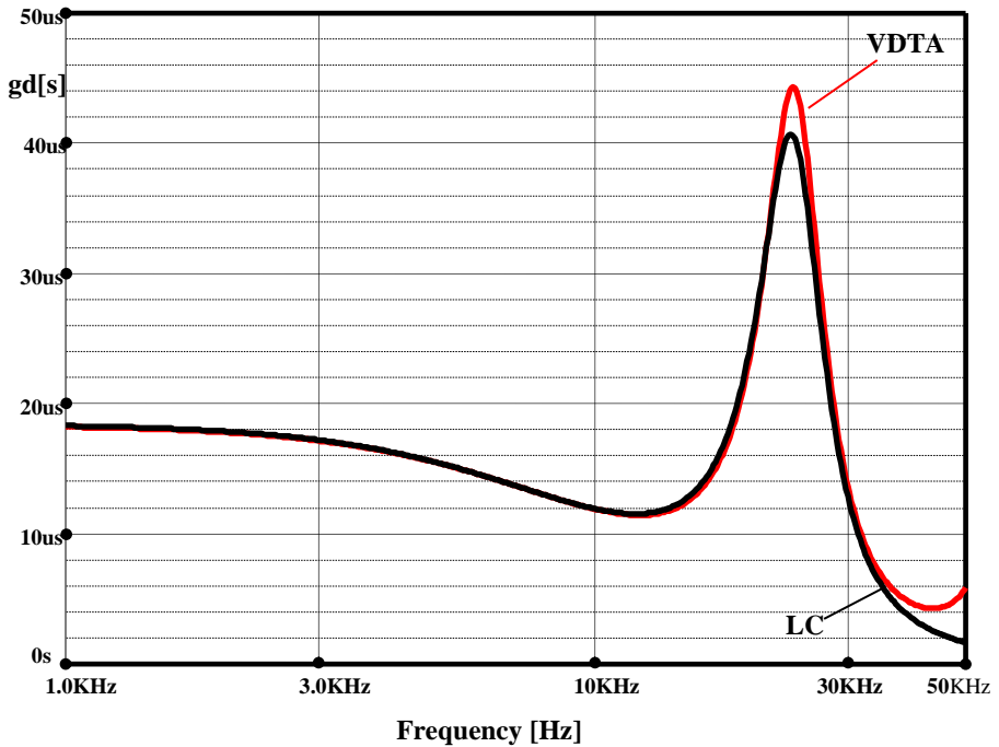
Fig. 6: The group delay response of ideal LC ladder and VDTA-based active filter.
