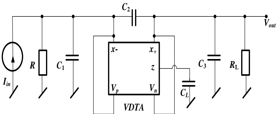
Fig. 4: Active implementation of the filter from Fig. 3.
