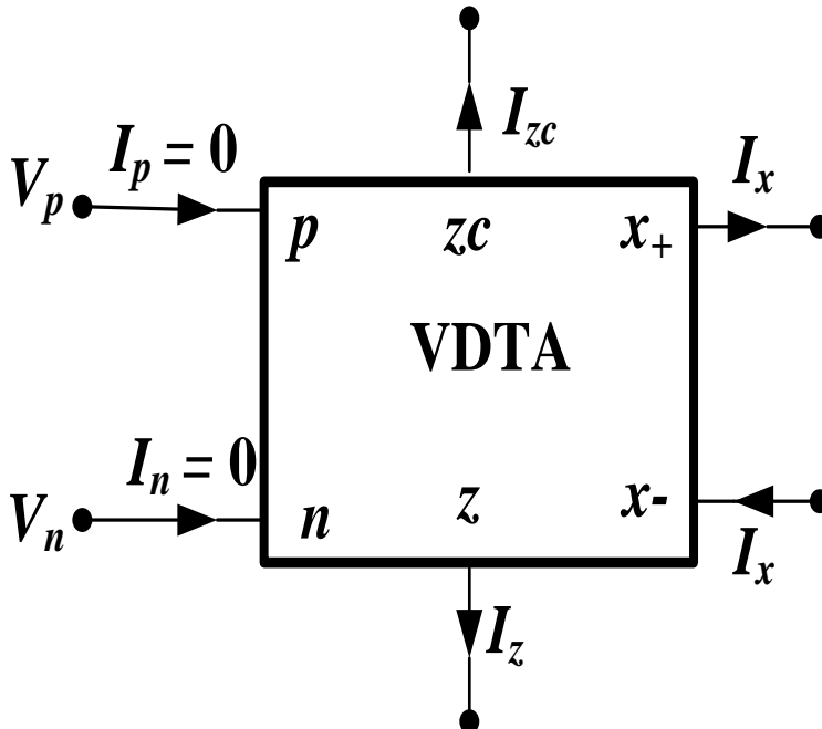
Fig. 1: Symbol of the VDTA
