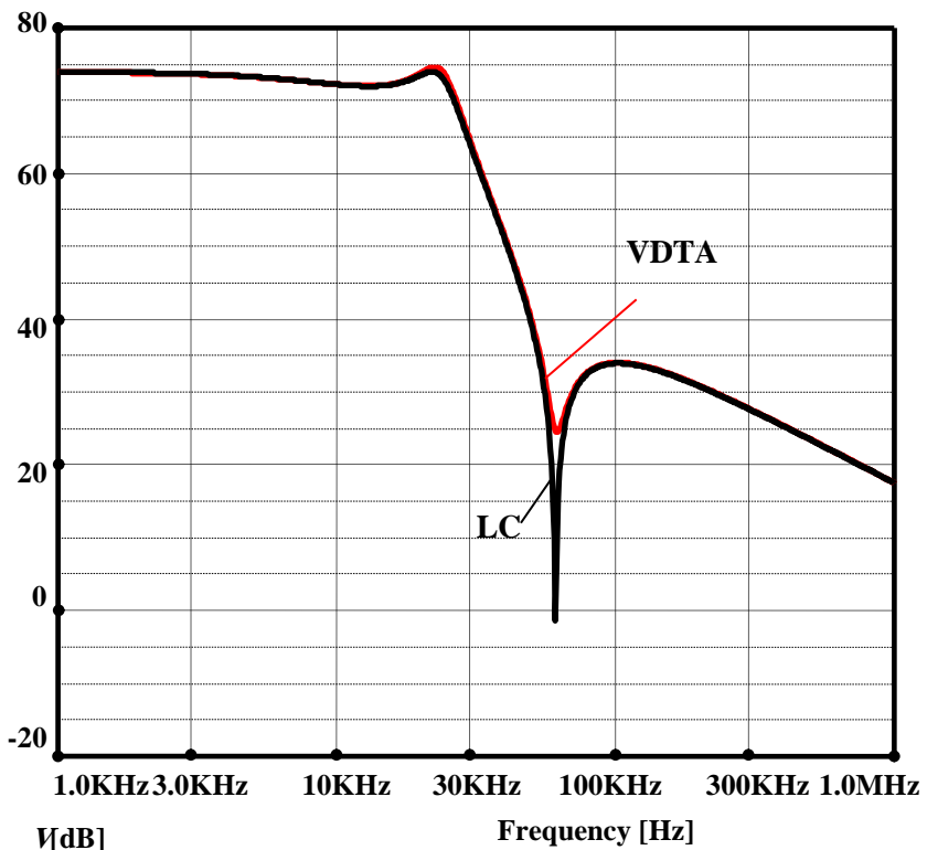
Fig. 5: The frequency responses of ideal LC ladder and VDTA-based active filter.
