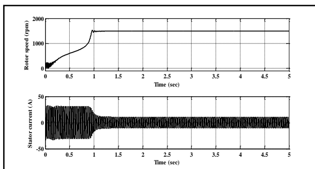
Fig. 3. A-phase stator current and rotor speed for normal operating condition
