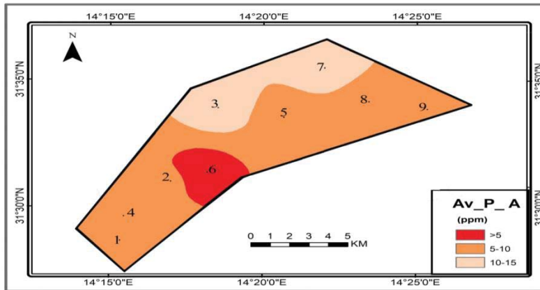
Fig. (9). The spatial distribution of available phosphorus (Av-P) in soil samples taken at depths of 20-40 cm in the study area.
