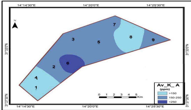
Fig. (10). The spatial distribution of available potassium (Av-K) in soil samples taken at depths ranging from 0 to 20 cm in the studied area
