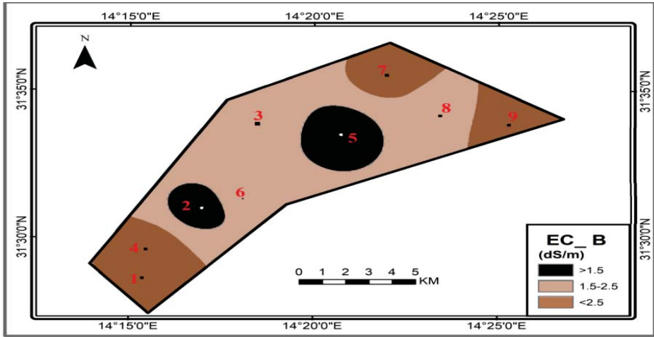
Fig.(5). Spatial variability within Ec values in the surface layer (20-40cm) of the studied soils.
