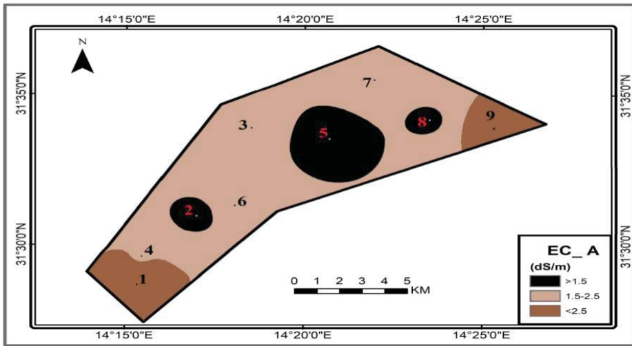
Fig. (4). Spatial variability within Ec values in the surface layer (0-20 cm) of the studied soils.
