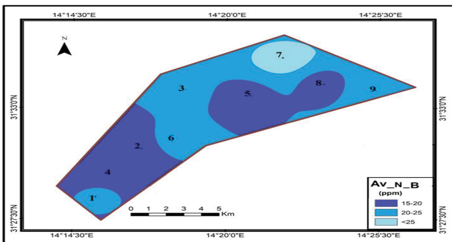
Fig. (6). The spatial distribution of available nitrogen (Av-N) in soil samples taken at depths ranging from 0 to 20 cm in the studied area.
