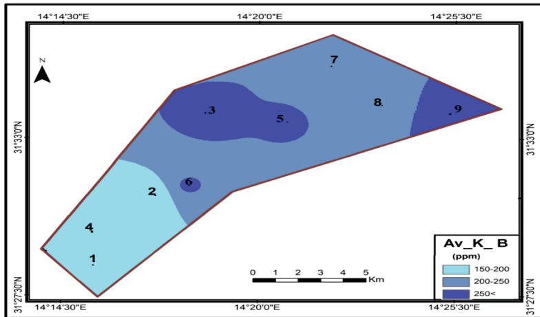
Fig. (10). The spatial distribution of available potassium (Av-K) in soil samples taken at depths ranging from 20 to 40 cm in the studied area.
