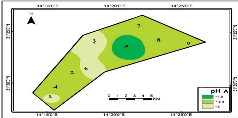
Fig. (2). There is spatial variability within pH values in the surface layer (0–20 cm) of the studied soils.
